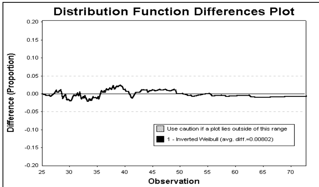
Figure 3: Distribution Function Differences Plot for the Processing-Time Data
