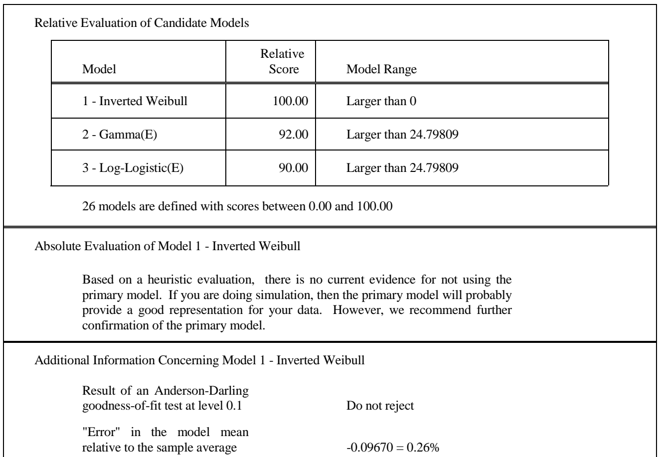
Figure 1: Evaluation of Candidate Models for the Processing-Time Data
