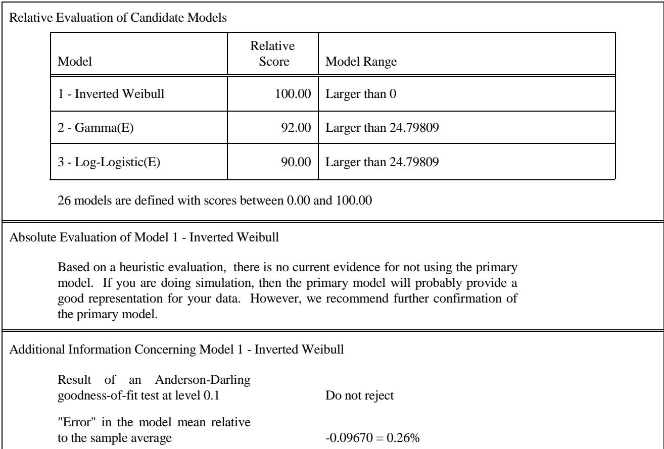
Figure 1: Evaluation of Candidate Models for the Processing-Time Data
