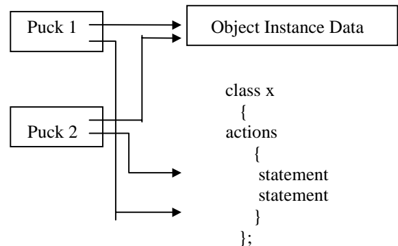
Figure 5: An Active Object With Two Pucks
