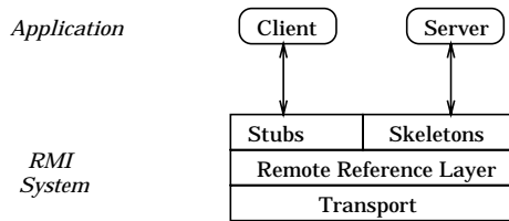
Figure 1: Java RMI Architecture
