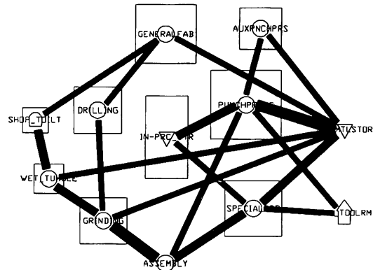
Figure 5. Activity Relationship Diagram
