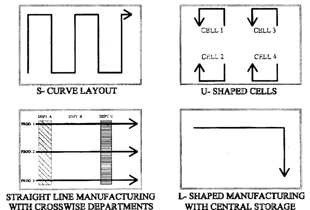
Figure 2. Layout Configurations
