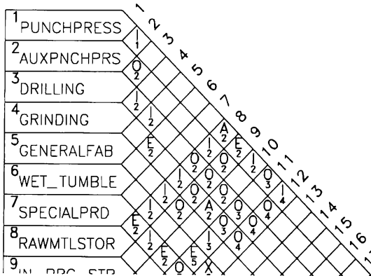
Figure 4. Activity Relationship Chart
