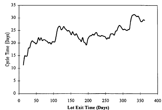
Figure 4: Cycle Time vs. Lot Exit Time for Run with Significant Initialization Bias
