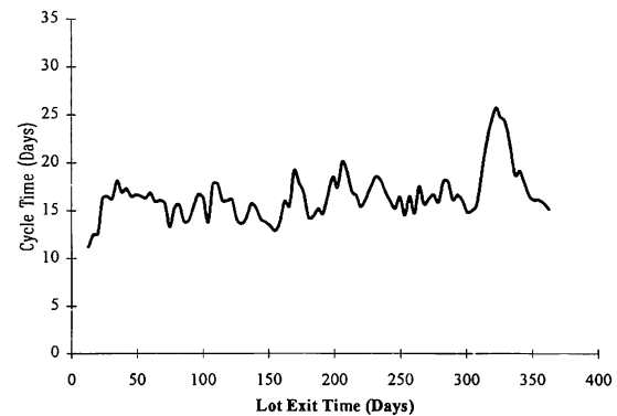
Figure 3: Cycle Time vs. Lot Exit Time for Run with Negligible Initialization Bias
