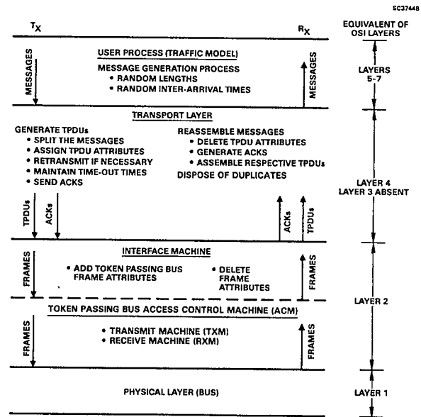
Fig. 4. Overview of the simulation model
