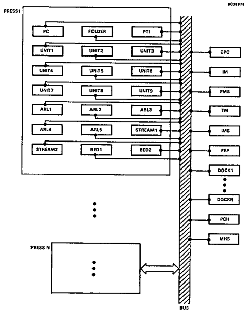
Fig. 2. Press-Station configuration
