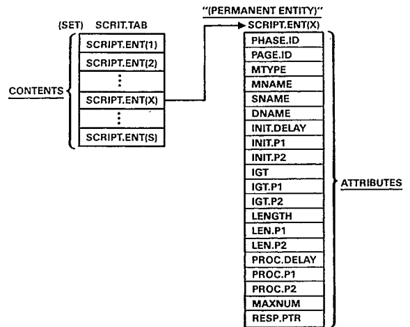
Fig. 9. Data Structures (contd.)
