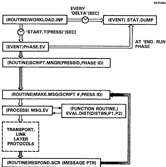
Fig. 7. Flowchart of the workload model
