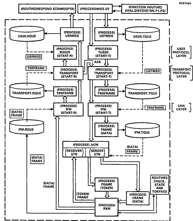
Fig. 6. Link and Transport layer protocols
