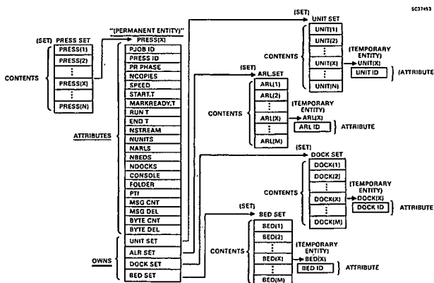
Fig. 8. Data Structures
