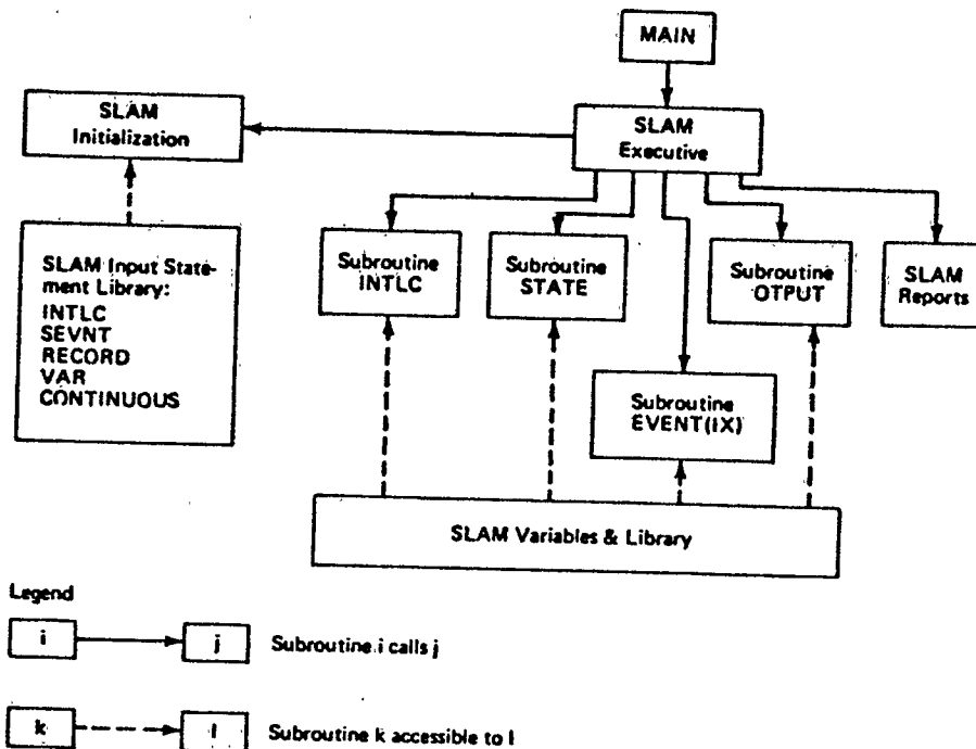
Figure 6. SLAM Organization for Continuous Modeling
