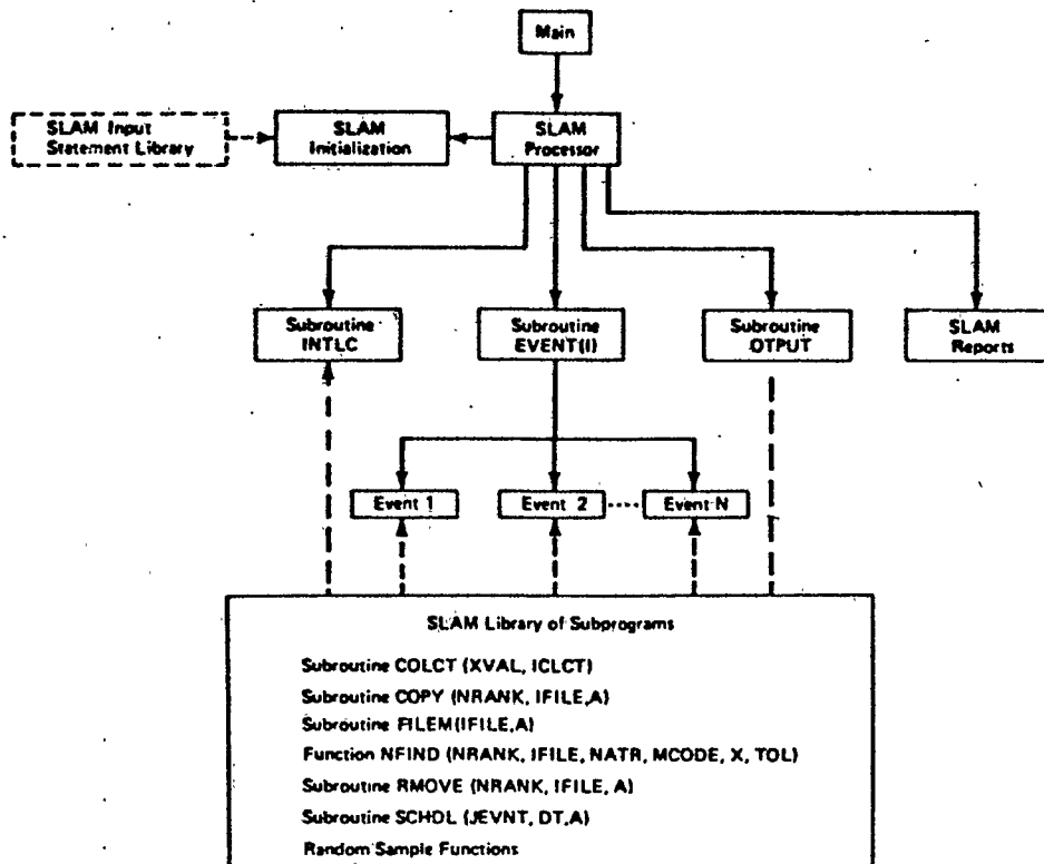
Figure 2. SLAM Organization for Discrete Event Modeling
