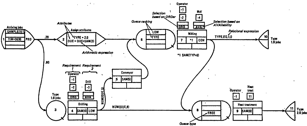
Figure 3 FLEXIBLE PRODUCTION DEPARTMENT NETWORK
