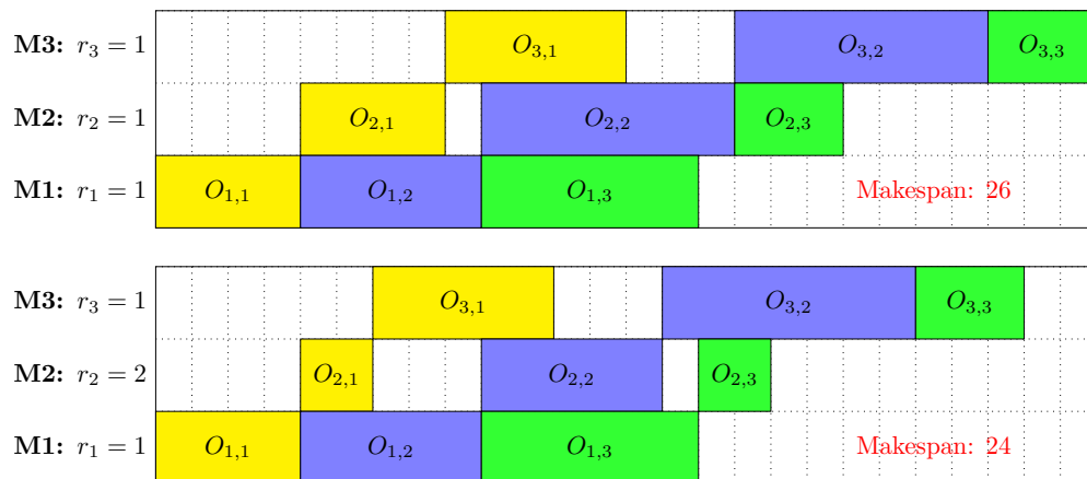
Figure 2: Difference in makespan with more resources assigned to machines.
