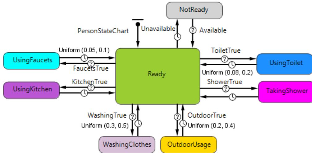
Figure 1: Person Statechart.
