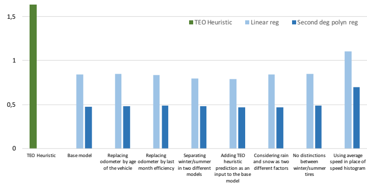
Figure 2: Consumption models.
