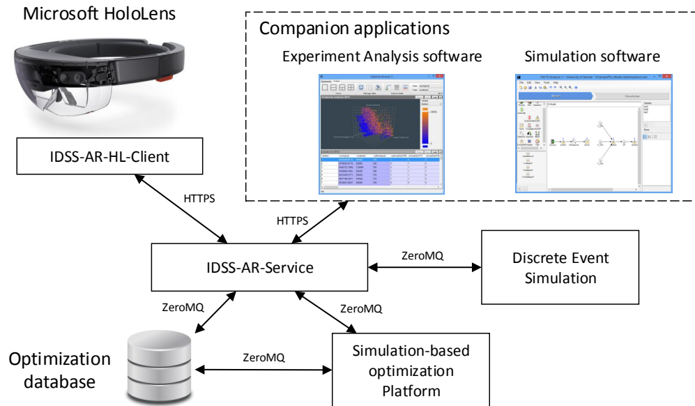
Figure 2: System architecture for IDSS-AR.
