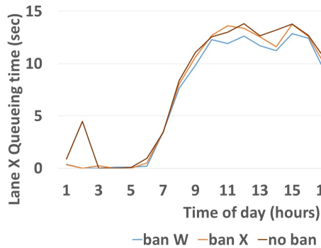
Figure 7: IC queue time in Lane X.
