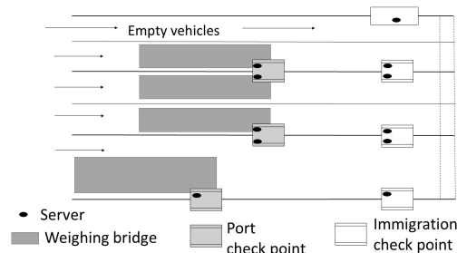
Figure 2: Layout of lanes at outbound gate.
