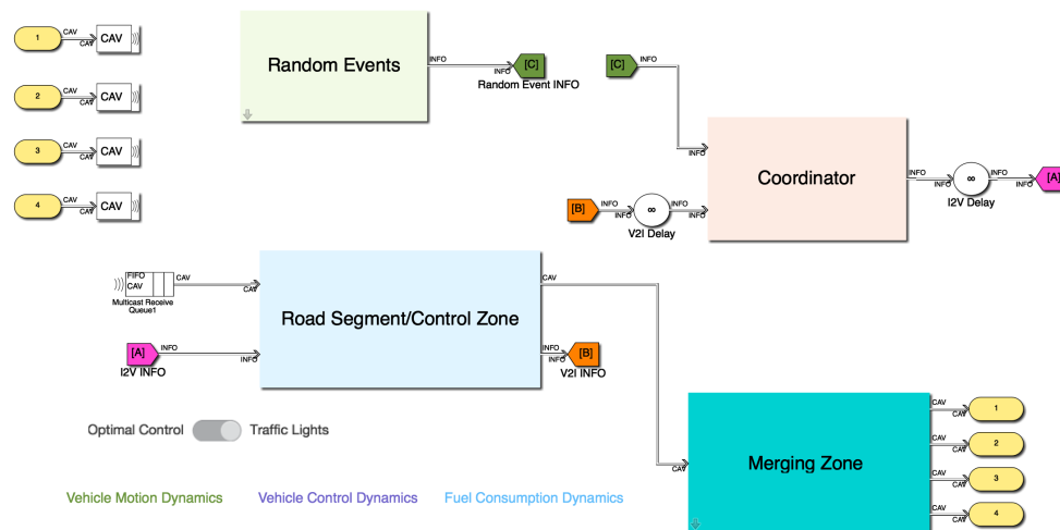
Figure 2: Simulink ® model of an intersection with four road segments (input/outputs).
