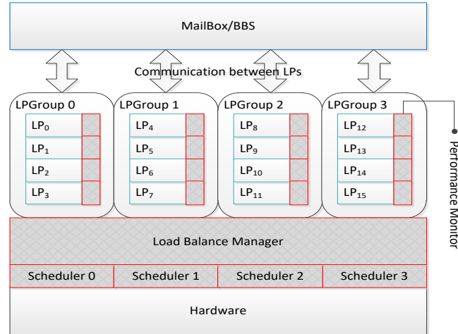
Figure 1: The architectural overview of WS-DLB algorithm on multicore platform.
