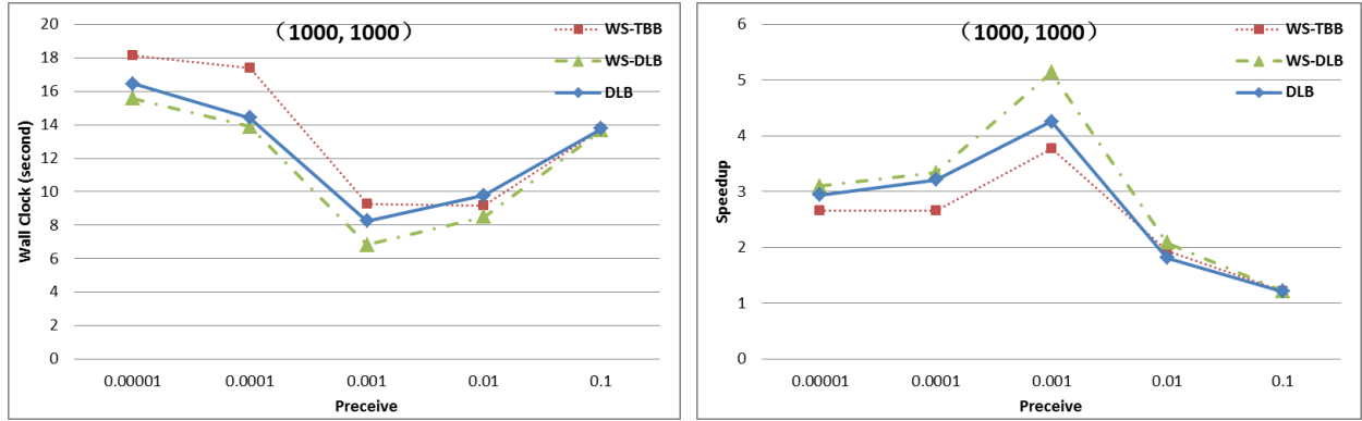
Figure 5: Performance Comparison of La-pdes using different p_{\text{receive}}
