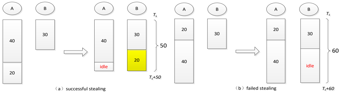
Figure 2: An example to show why scheduling sequence affects the work-stealing under the same workload distribution
