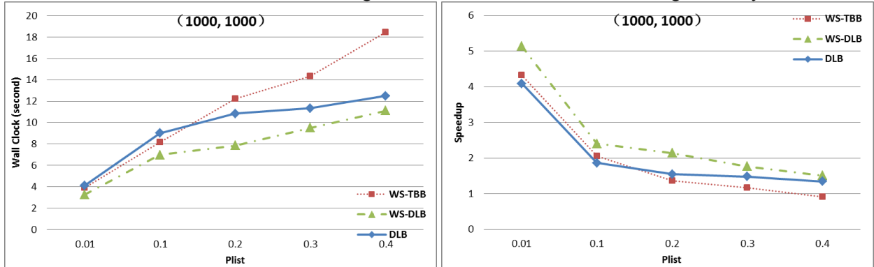
Figure 4: Performance Comparison of La-pdes using different p_{list}
