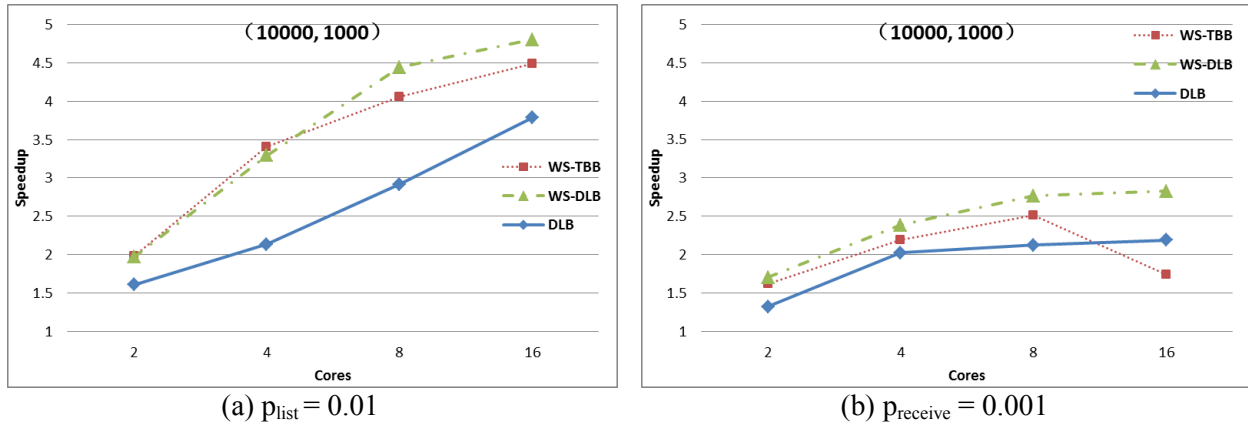
Figure 6: Performance Comparison of La-pdes using different cores
