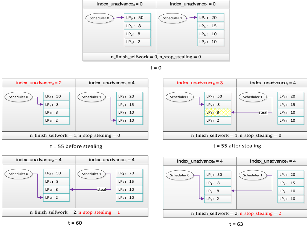
Figure 3: an example to show the procedure of the work-stealing scheme
