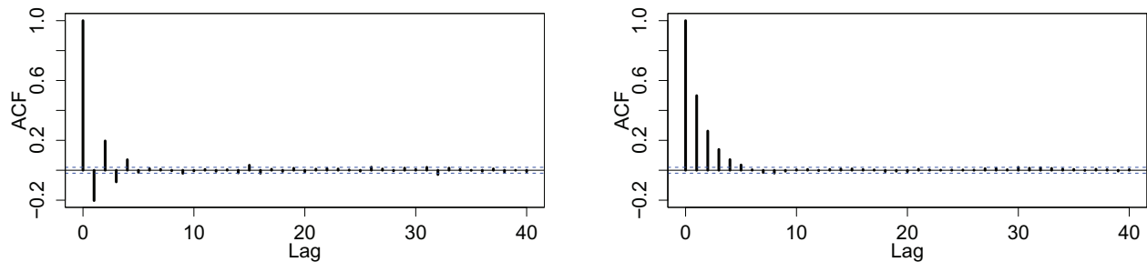
Figure 1: Autocorrelation function of two time series—horizontally dashed: significance band (95%).
