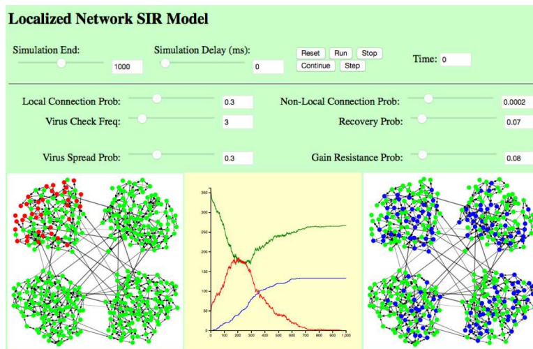
Figure 3: A collage of visual components of a Nova Online ‘SIR epidemic on small-world networks’ online app. Sliders in the top panel permit the density of connections within local clusters and the sparsity of connections among these clusters to be manipulated, as well as setting parameters that control rates of transmission, recovery and levels of resistance after recovery to be set. The lower left and right panels illustrate the initial and final (in this case after 1000 time iterations) states of the simulation (S: green; I: red; R: resistant) while the course of the epidemic is plotted (same color codes) over time.
