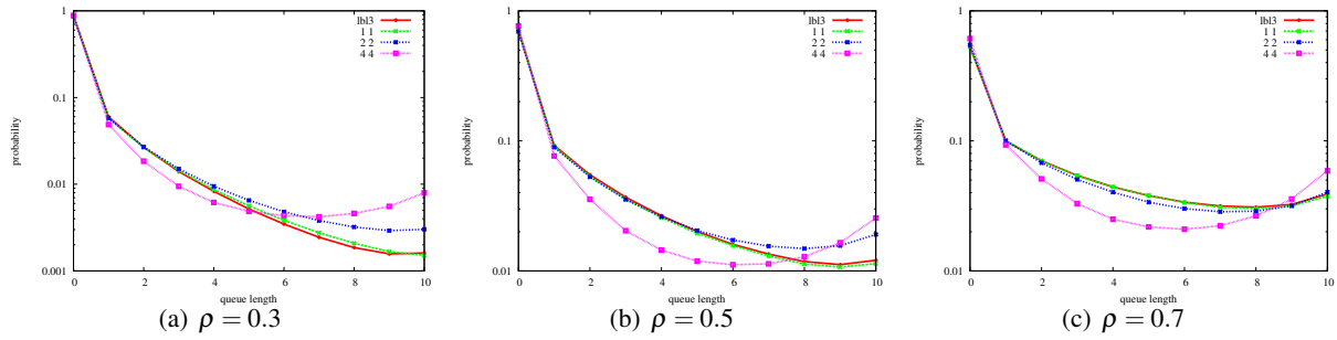
Figure 5: Queue length distribution for the trace LBL-TCP-3 and different CAPP(25, \cdot, \cdot) .
