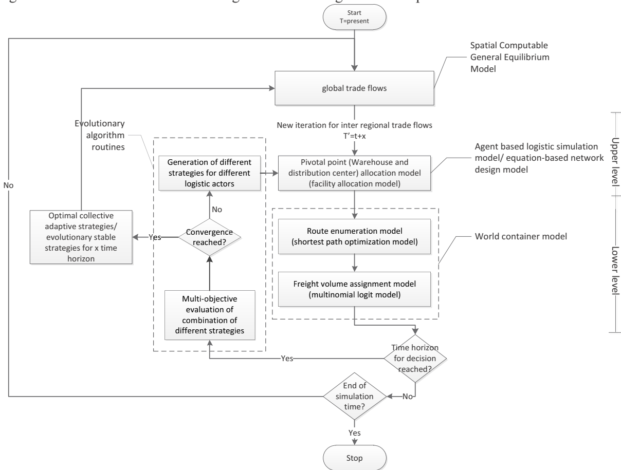
Figure 4 Computational framework
