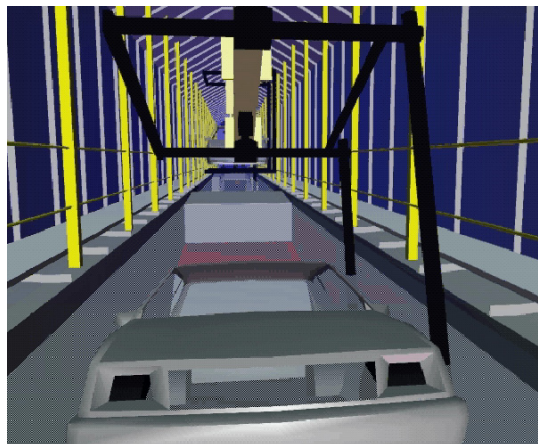
Figure 9: Emulation exhaustively tests control systems
