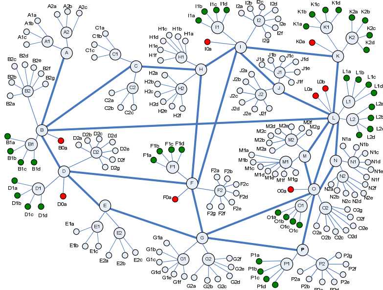
Figure 2: Three Tier Topology with 16 Backbone Routers (A-P), 32 Point of Presence Routers (A1-P2) and 170 Access Routers (A1a-P2g) – 8 red and 40 green Access Routers may operate at different speeds
