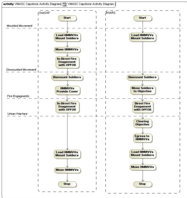
Figure 3: Activities in OneSAF and IWARS
