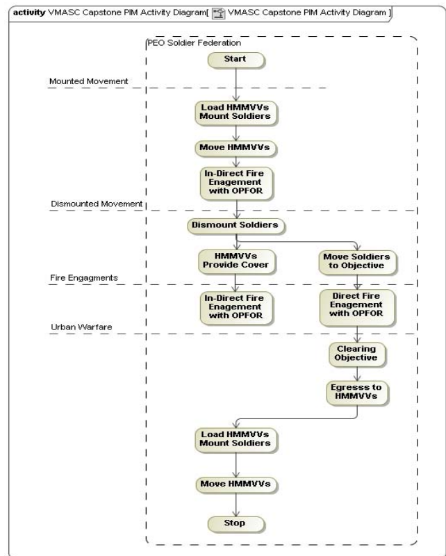
Figure 1: Activity Diagram
