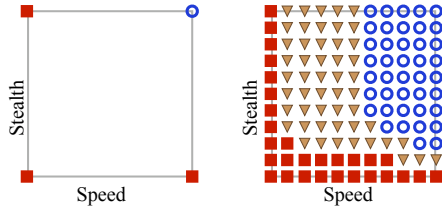
Figure 4: 2^2 and 11^2 factorial designs for capture-the-flag.
