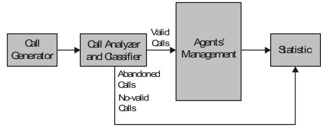
Figure 3: Block diagram of the simulation model of the predictive dialer.
