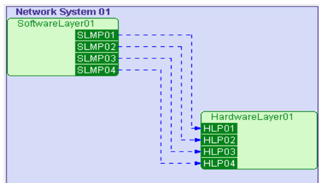
Figure 10: SoftwareLayer01 to HardwareLayer01 mapping.
