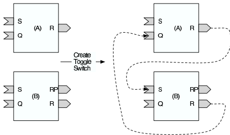
Figure 4: Iconified Toggle Switch
