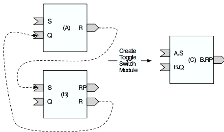
Figure 5: Iconified Toggle Switch with Input/Output Ports
