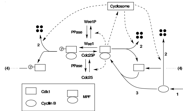
Figure 1: Pathway Diagram for the Frog Egg Cell Cycle
