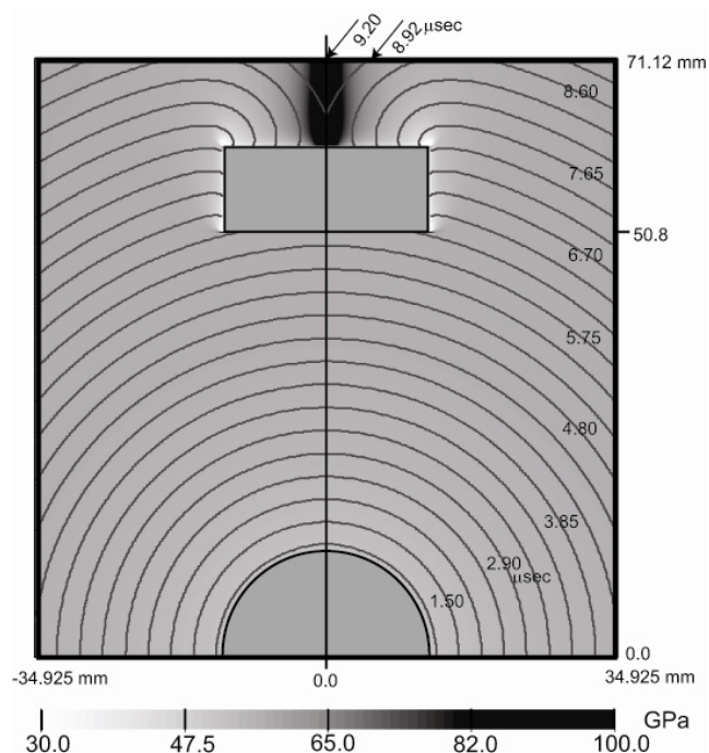
Figure 6: Isochronal Contours for the DSD-Based Motion Rule Model of the Passover Experiment.
