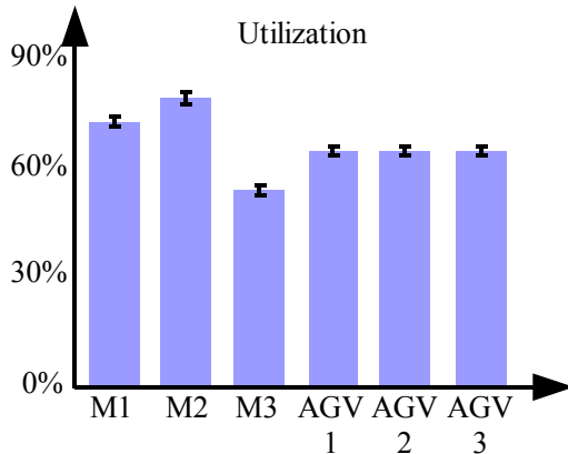
Figure 2: Utilization
