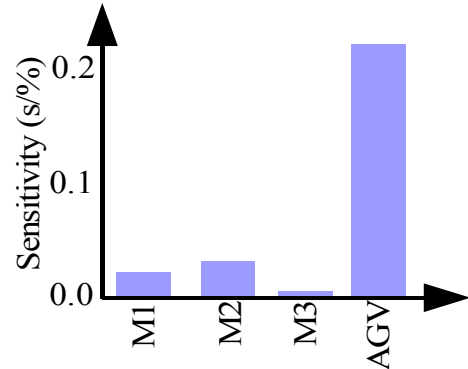
Figure 8: Measured Machine Sensitivities
