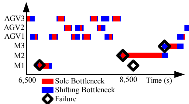
Figure 6: Bottlenecks and Machine Failures
