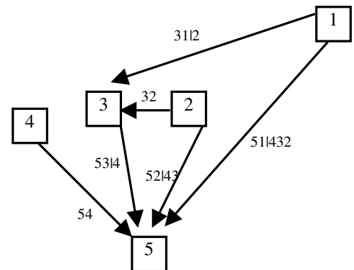
Figure 28: BN with Conditional Correlations Corresponding to Example 8
