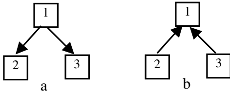
Figure 4: A Simple Example Of BN's
