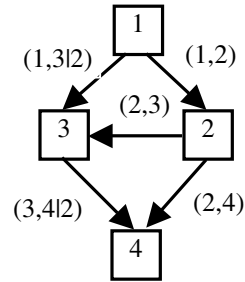
Figure 20: Example 4; BN with Conditional Correlations
