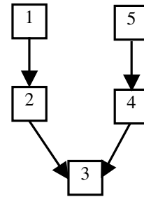
Figure 29: BN Corresponding To Example 9
