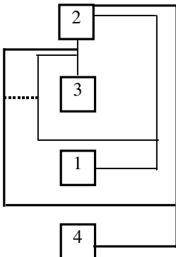
Figure 19: Example 4; Step 2,3,4 with C-Vine
