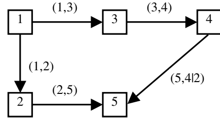
Figure 15: Example 2; BN with Conditional Correlations
