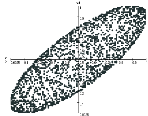
Figure 3: The Scatter Plot of the Elliptical Copula with Correlation 0.8
