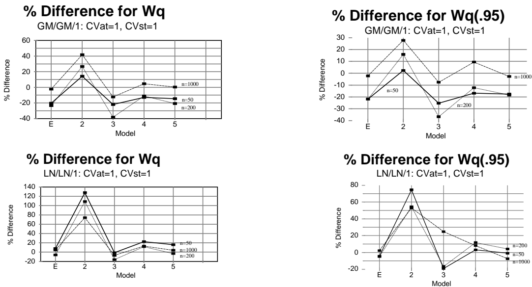
Figure 1: CV_{at} = 1, CV_{st} = 1 .
