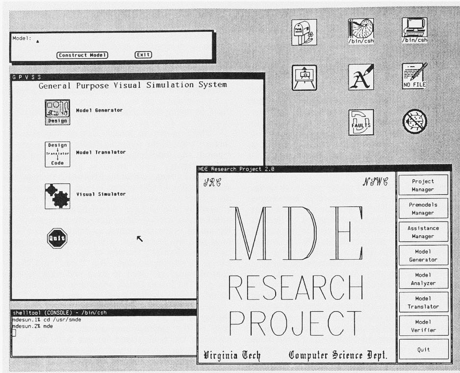
Figure 1. GPVSS Top-Level Window and Activation of Model Generator
