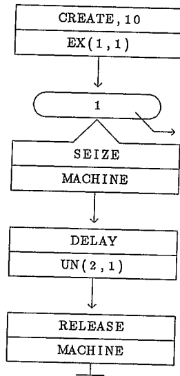
Figure 2: Block Diagram for Simple System
