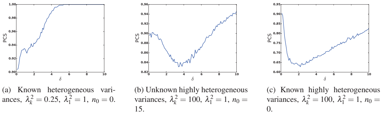
Figure 1: The PCS of the BIZ procedure versus \delta for three different slippage configurations with 100 alternatives and P^* = 0.9 . We observe in all three examples that the PCS converges to P^* as \delta goes to 0. The first example (a) shows typical behavior, where the PCS is above P^* for all values of \delta . The second (b) and third (c) examples are atypical, and were chosen specially to illustrate that BIZ can underdeliver on PCS in slippage configurations when n_0 is small and the variance of the best alternative is much larger than the variance of the other alternatives.
