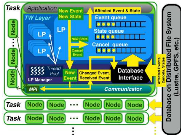
Figure 9: Cloning affected events and states in repeating execution.
