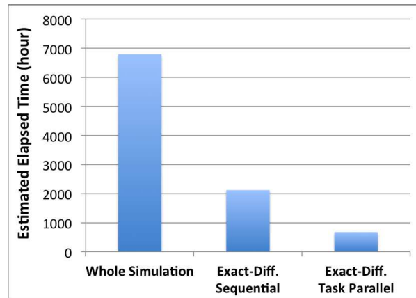
Figure 11: Estimated elapsed time of 161K times repeating execution with 192 cores.
