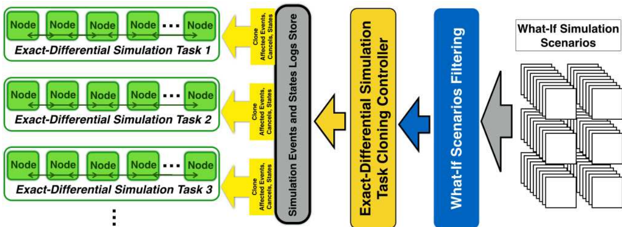
Figure 4: Overview of large-scale what-if simulation with exact-differential simulation.
