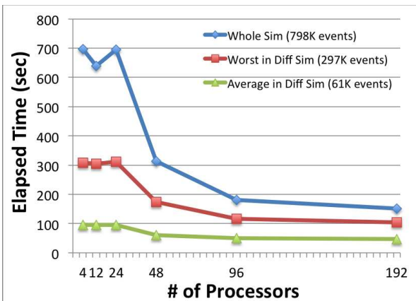
Figure 10: Strong scale in our previous work (Hanai, et al. 2015).
