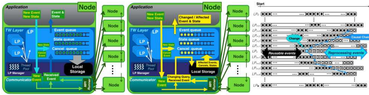
Figure 1: Initial execution. Figure 2: Repeating execution. Figure 3: Reprocessing events.
