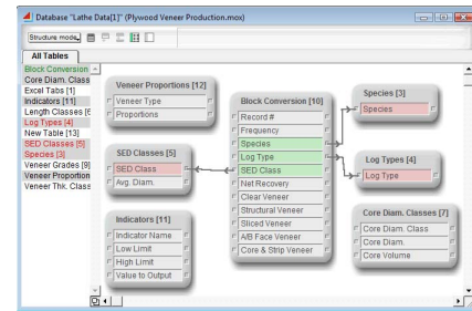
Figure 7: ExtendSim database structure
