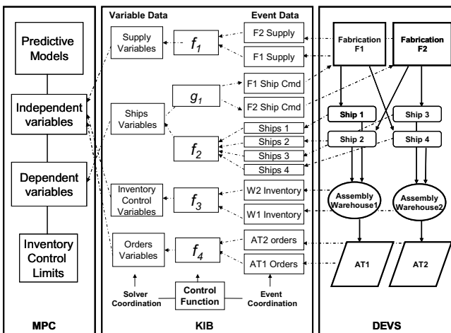
Figure 4. Composition of DEVS and MPC with KIB
