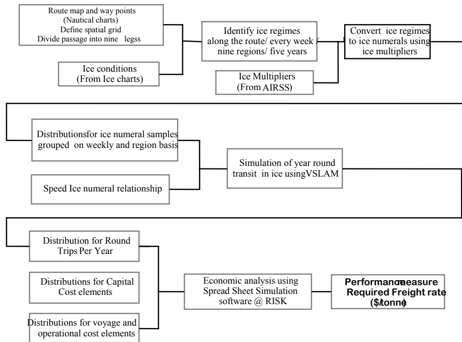
Figure 2: Flow Chart of Simulation of Ship Passage through the Northwest Passage
