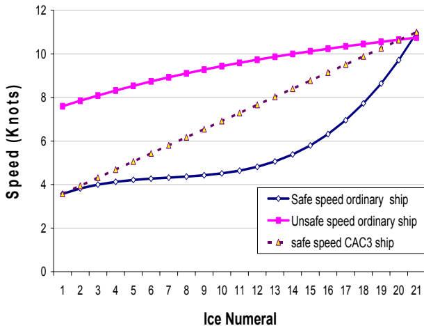
Figure 3: Ship Speed as a Function of Ice Numeral.
